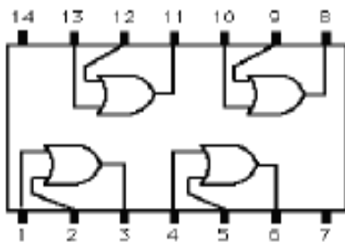
7432 Quad 2-Input OR Gate
