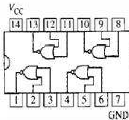
7402/74LS02
